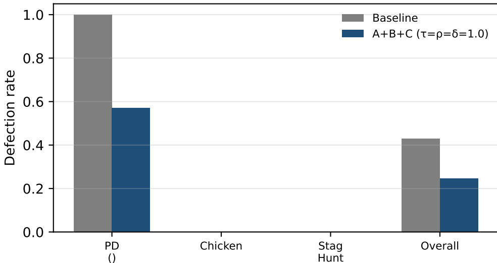
F3: Defection rate — baseline vs. A+B+C GT-HarmBench social-dilemma subset
