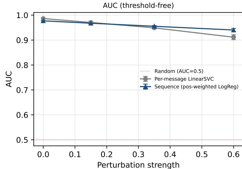
Discourse-noise perturbation sweep — PAN 2012 (positives perturbed, negatives clean; 5 seeds)
