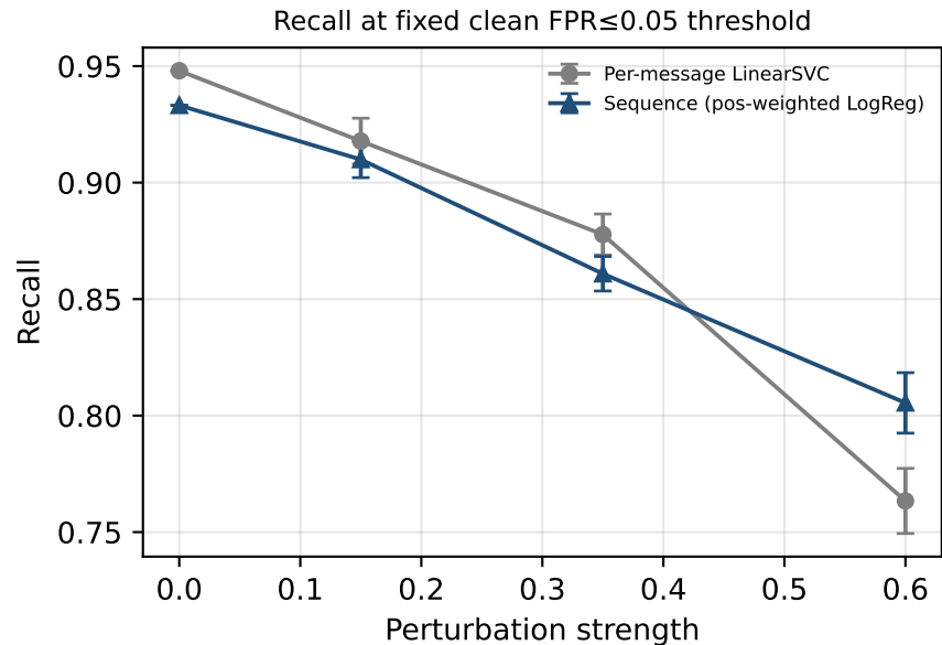
Discourse-noise perturbation sweep — PAN 2012 (positives perturbed, negatives clean; 5 seeds)
