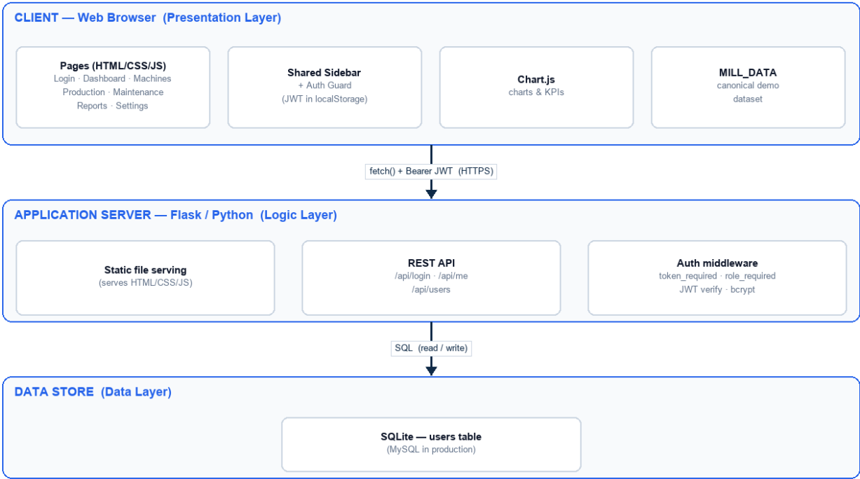
System Architecture — Smart Paper Mill Production Monitoring Dashboard
