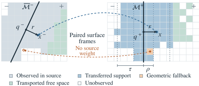
Source TSDF
