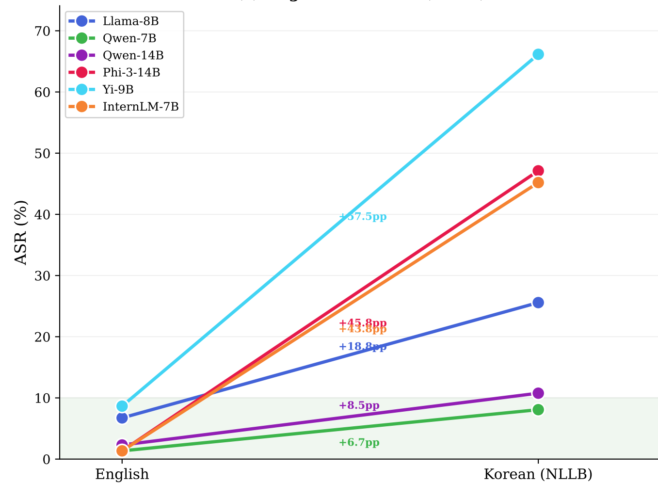
(a) English → Korean (NLLB)
