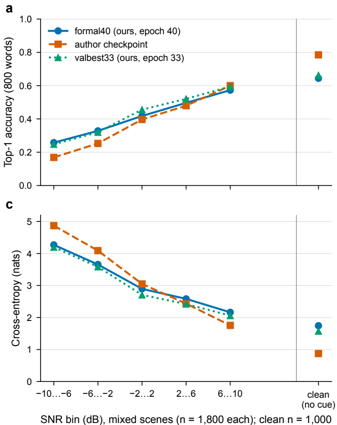
Correct-cue performance on the frozen 10,000-trial bank (Job 728520; point estimates)
