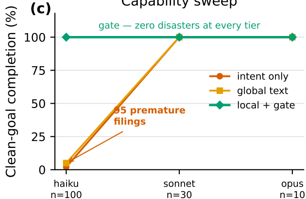
(c) Capability sweep
