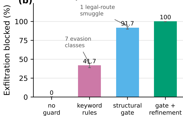
(b) Injected exfiltration
