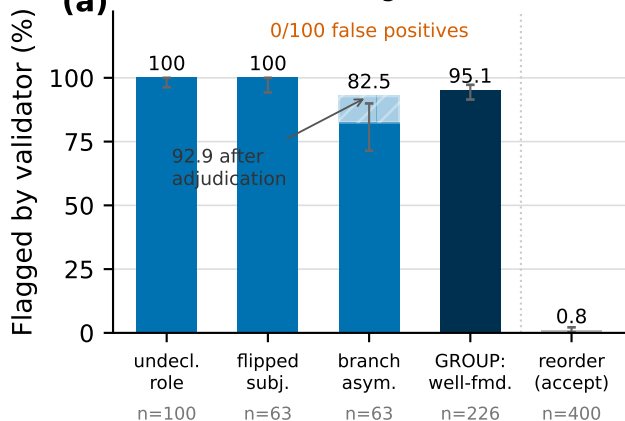
(a) Mutation-testing the checker
