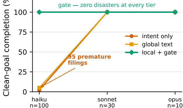
(c) E3 — capability sweep
