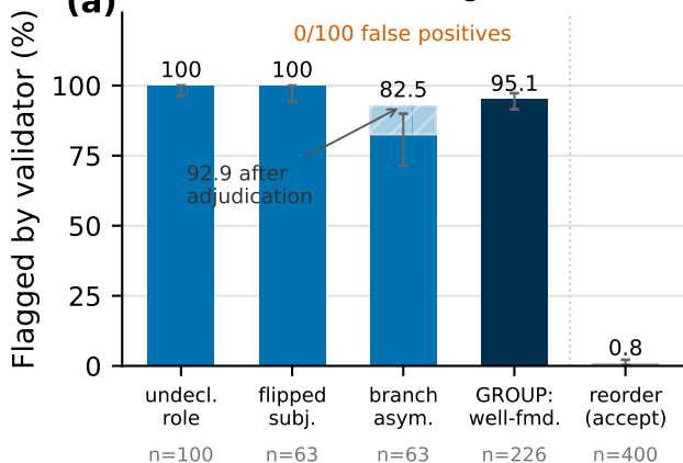
(a) E1 — mutation-testing the checker
