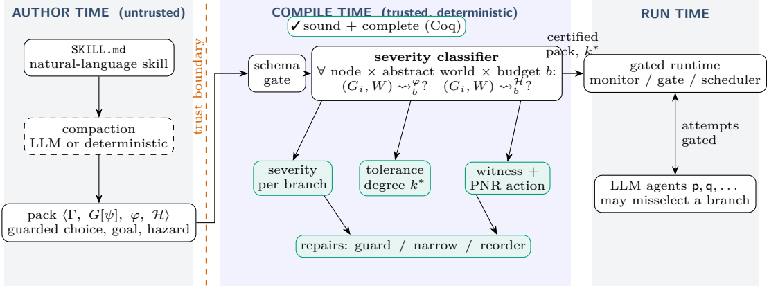
■ Figure 2 Architecture. Compaction from prose to a pack is untrusted and may use a language model; nothing beyond the trust boundary does. The severity classifier runs the discipline’s existing reachability search pointwise at every branch of every choice, at every abstract world and budget, and emits a per-branch severity, the tolerance degree k^* , a witness naming the point-of-no-return action, and repair suggestions. The certified pack drives the gated runtime that refuses out-of-protocol attempts.
