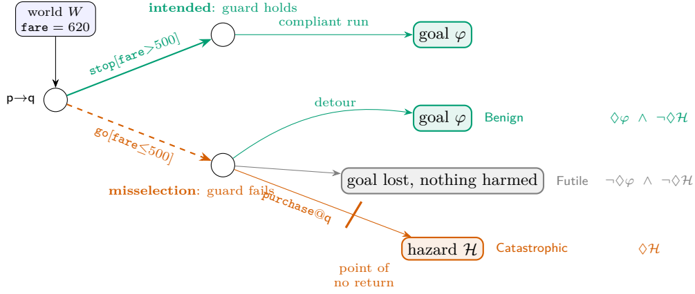
■ Figure 1 The idea. At a guarded choice in world W , the branch whose guard holds is intended ; taking the other is a misselection . Its severity is a property of the residual: Benign if the goal is still reachable, Futile if the goal is lost but no hazard is reachable, Catastrophic if a hazard is reachable — typically by crossing a point of no return , an irreversible capability after which the goal cannot be recovered.
