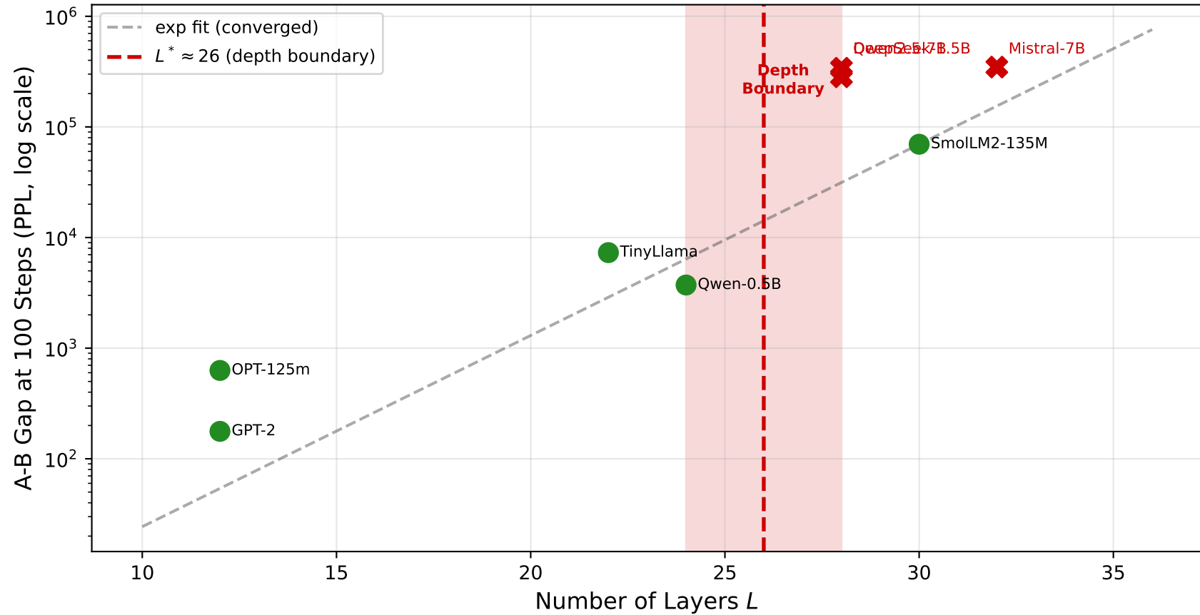
Figure 3: Depth Scaling — A-B Gap vs Model Depth
