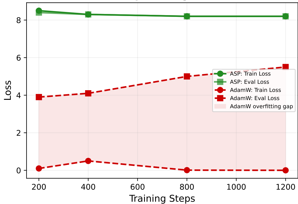
(b) ASP Implicit Regularization
