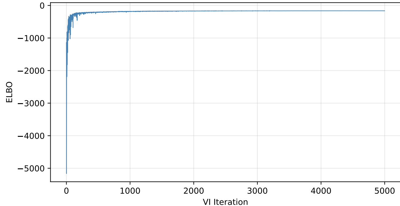
ELBO Convergence (Stochastic Gradient VI)
