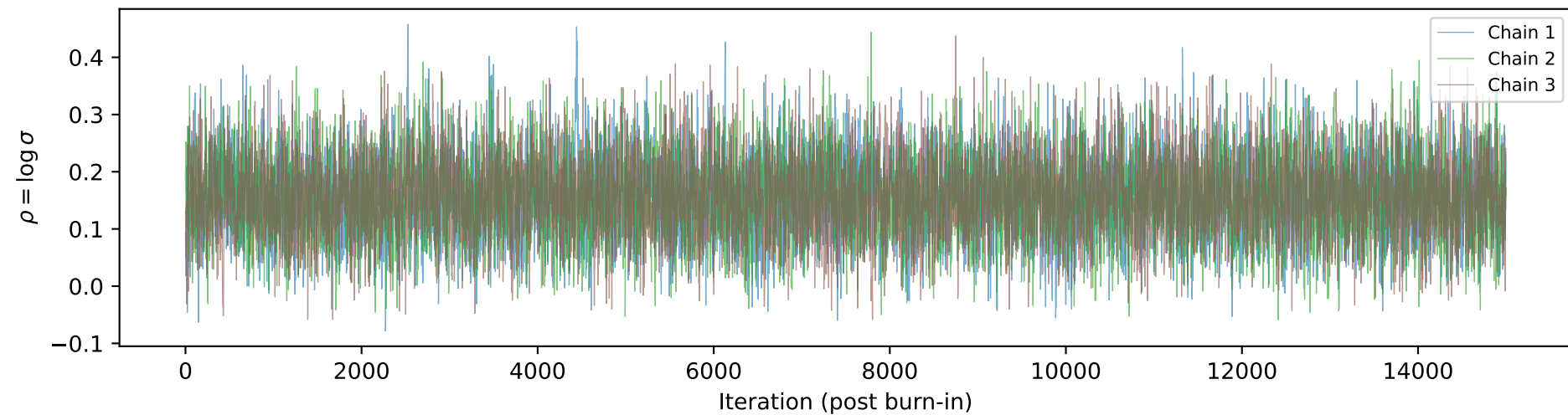
Trace plot — \rho = \log \sigma
