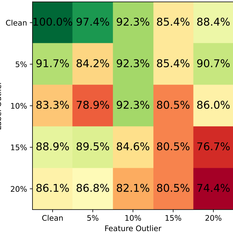
SKiP-multiply
