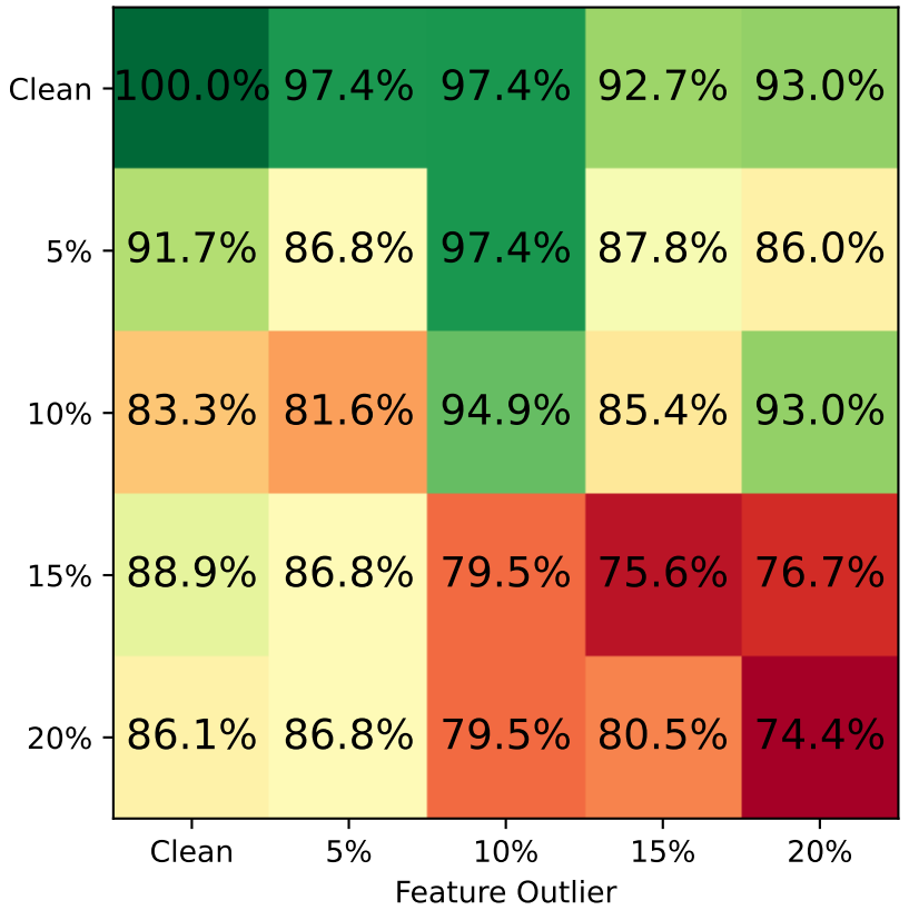
SKiP-average
