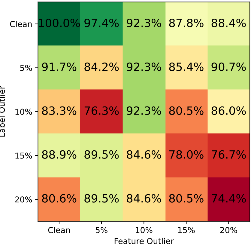
SKiP-minmax-multiply
