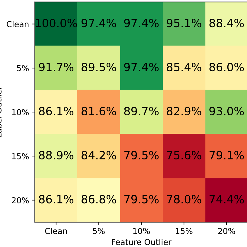
SKiP-minmax-average
