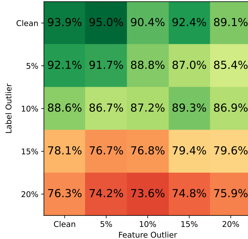
SKiP-minmax-average
