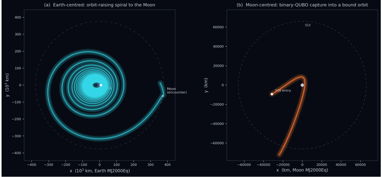
Figure 2: The full SMART-1-class mission reproduced in GMAT as a single continuous trajectory (real DE405 ephemerides, from the published GTO). (a) Earth-centred inertial view: continuous Hall thrust raises the apogee from GTO out to lunar distance (dashed ring = the Moon’s orbit), delivering the spacecraft to the lunar encounter after 140 d at 100 % duty. (b) Moon-centred view: the binary-QUBO anti-tangential schedule brakes the near-parabolic arrival inside the lunar sphere of influence (dashed) into a bound orbit. One uninterrupted propagation — no phase seam between spiral and capture.
