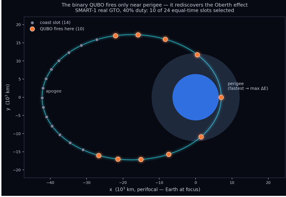
Figure 3: Under a 40 % duty constraint the binary optimizer rediscovers the Oberth strategy. Of N = 24 equal-time slots on SMART-1’s real GTO it selects the K = 10 of largest measured energy gain — exactly the slots straddling perigee, where the spacecraft is fastest ( dE = v dv ) — while the coast slots fall at apogee. No orbital mechanics is built in; the perigee-thrust policy emerges from the discrete optimization. Earth is shown to scale at the focus.
