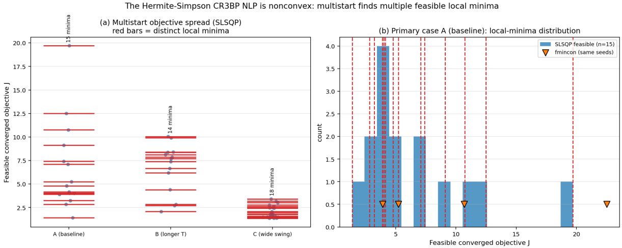
Figure 3: The Hermite–Simpson energy-optimal CR3BP transcription is nonconvex. Left : for three boundary-condition cases, the feasible converged objectives of 32 random multistarts (SLSQP); red bars mark distinct local minima. Nearly every feasible start reaches a different minimum, and the objective spread exceeds an order of magnitude. Right : primary case A, the distribution of feasible SLSQP minima (bars) with MATLAB fmincon results from the same seeds overlaid (orange triangles). The two optimisers scatter across the same multi-basin landscape — fmincon even reaches a minimum beyond the SLSQP range — but coincide to machine precision when seeded into a shared basin.
