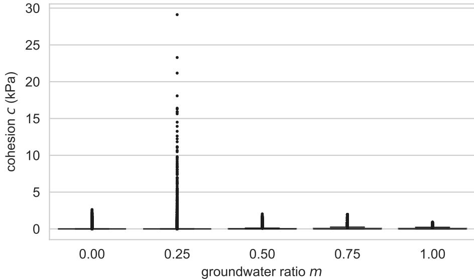
Inferred cohesion across the pore-pressure sweep
