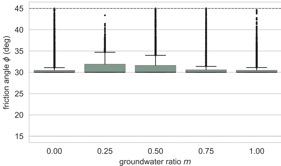
Inferred friction angle across the pore-pressure sweep
