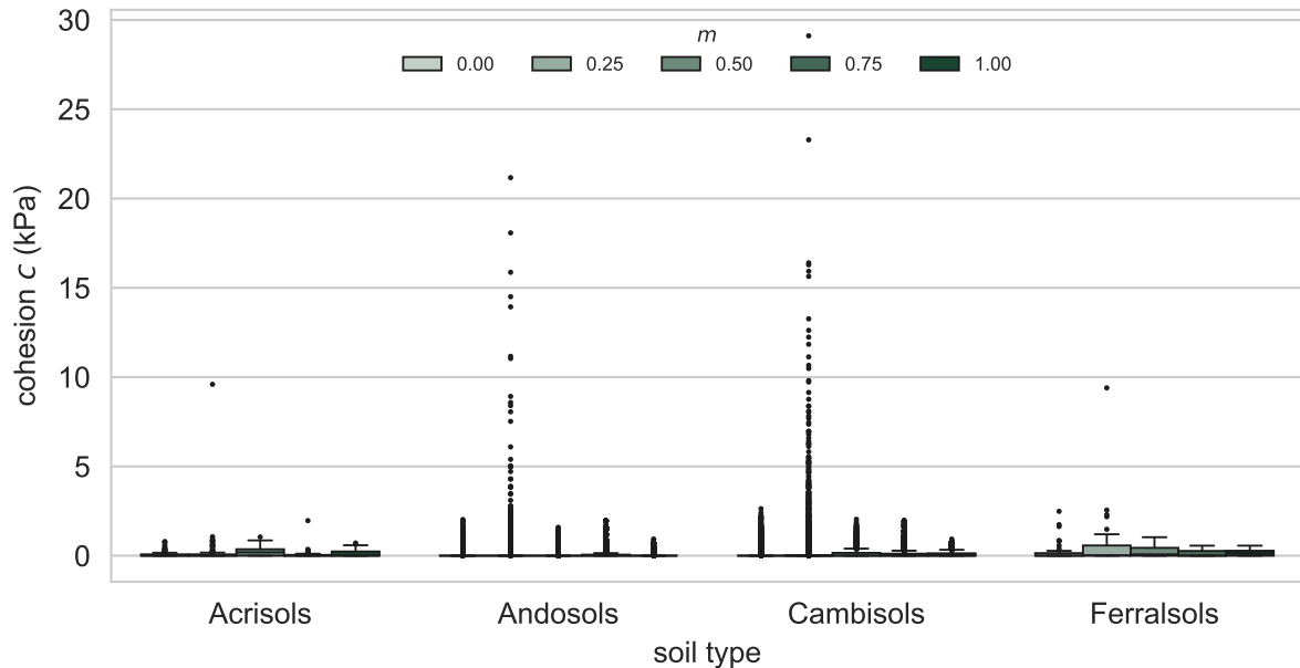
Inferred cohesion by soil type across the pore-pressure sweep
