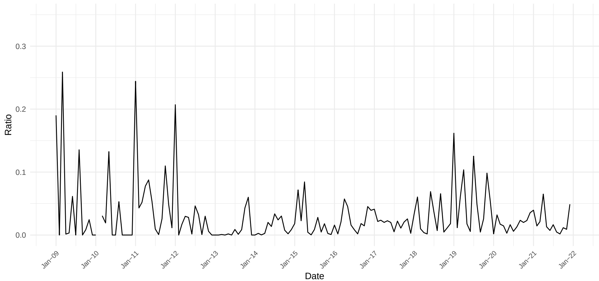
Estimated number of deaths and missing migrants over the sum of arrivals and pushbacks in the CMR
