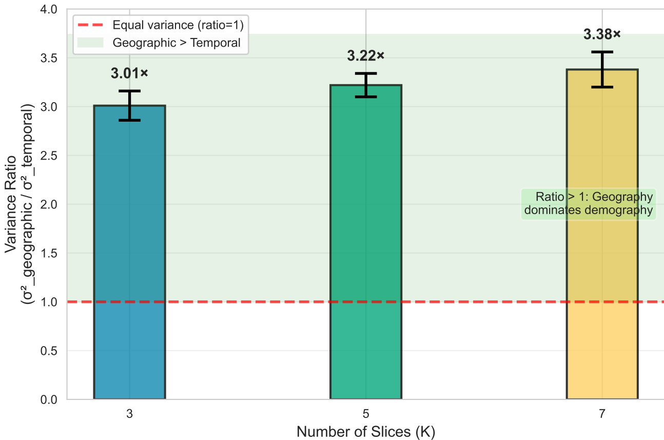
MAUP Sensitivity: Variance Ratio Across Slice Counts
