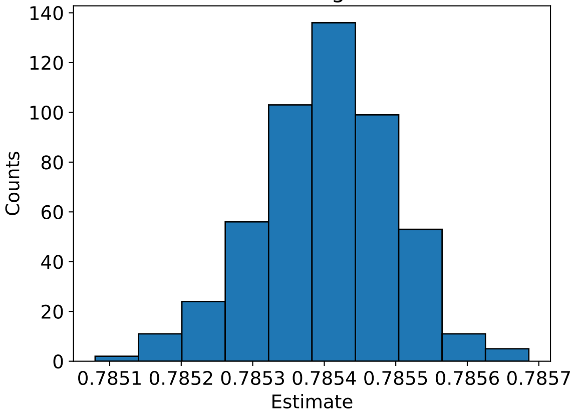
MC histogram
