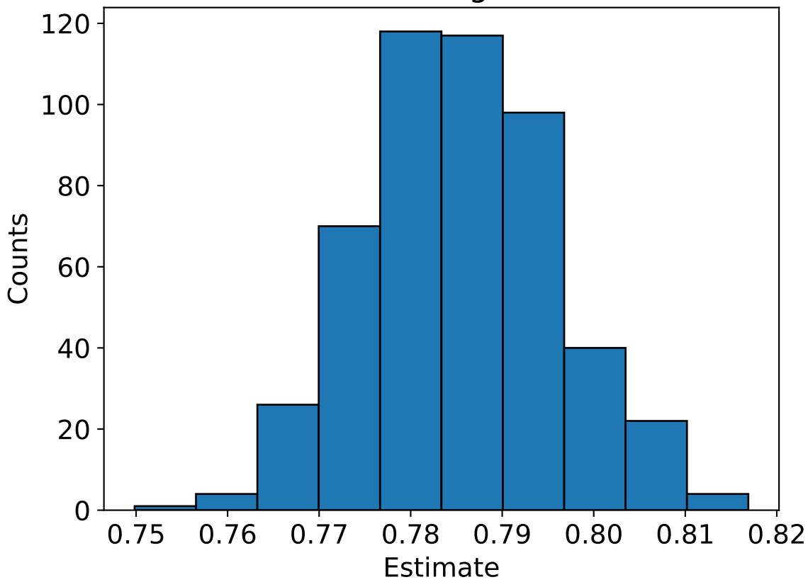
MC histogram
