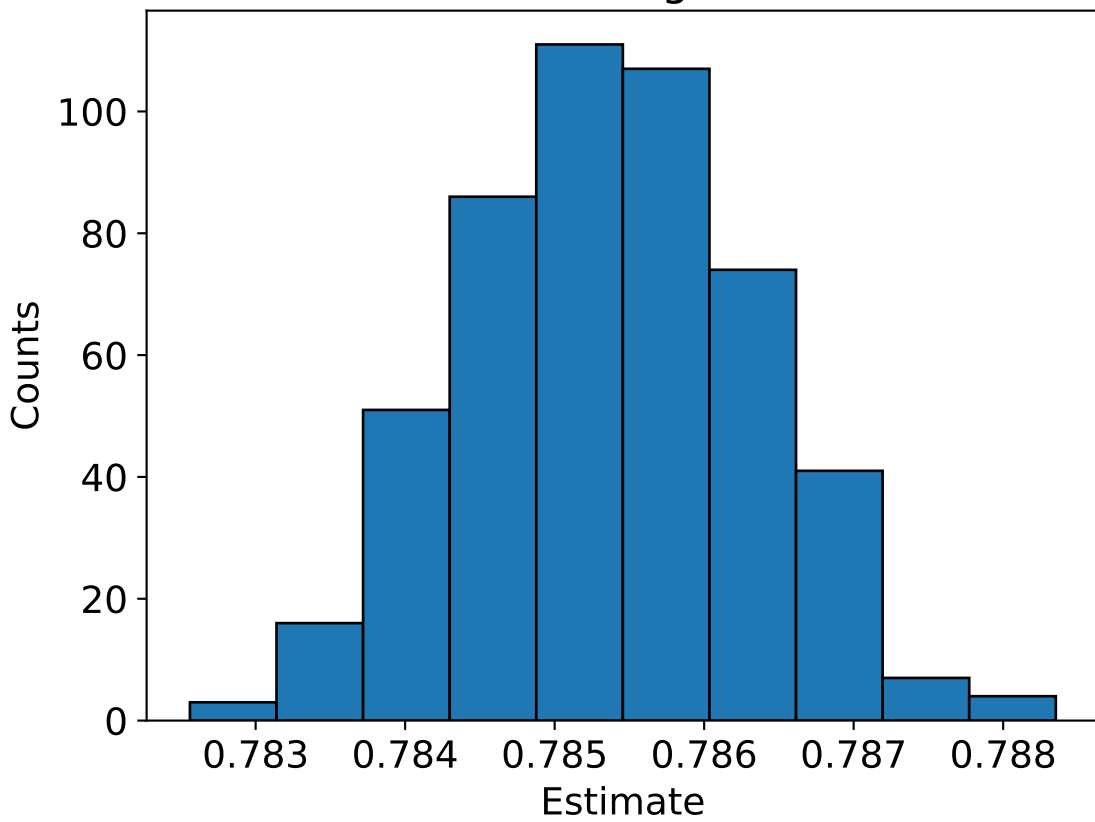
MC histogram
