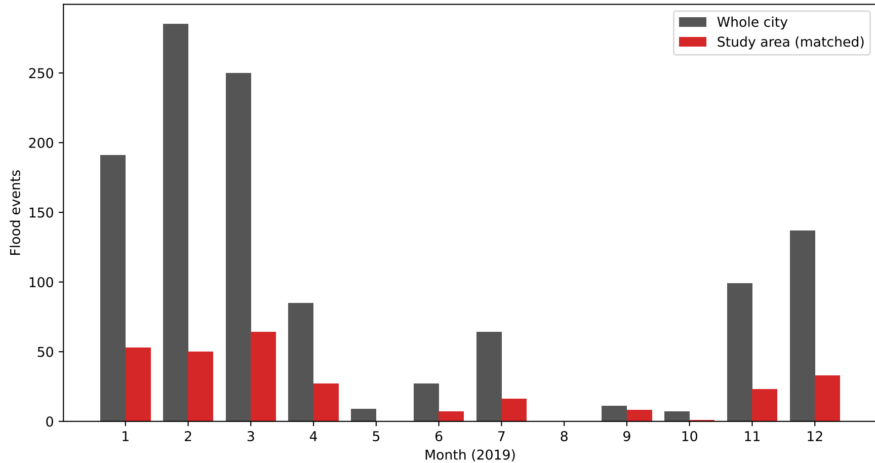
Seasonality of flood events
