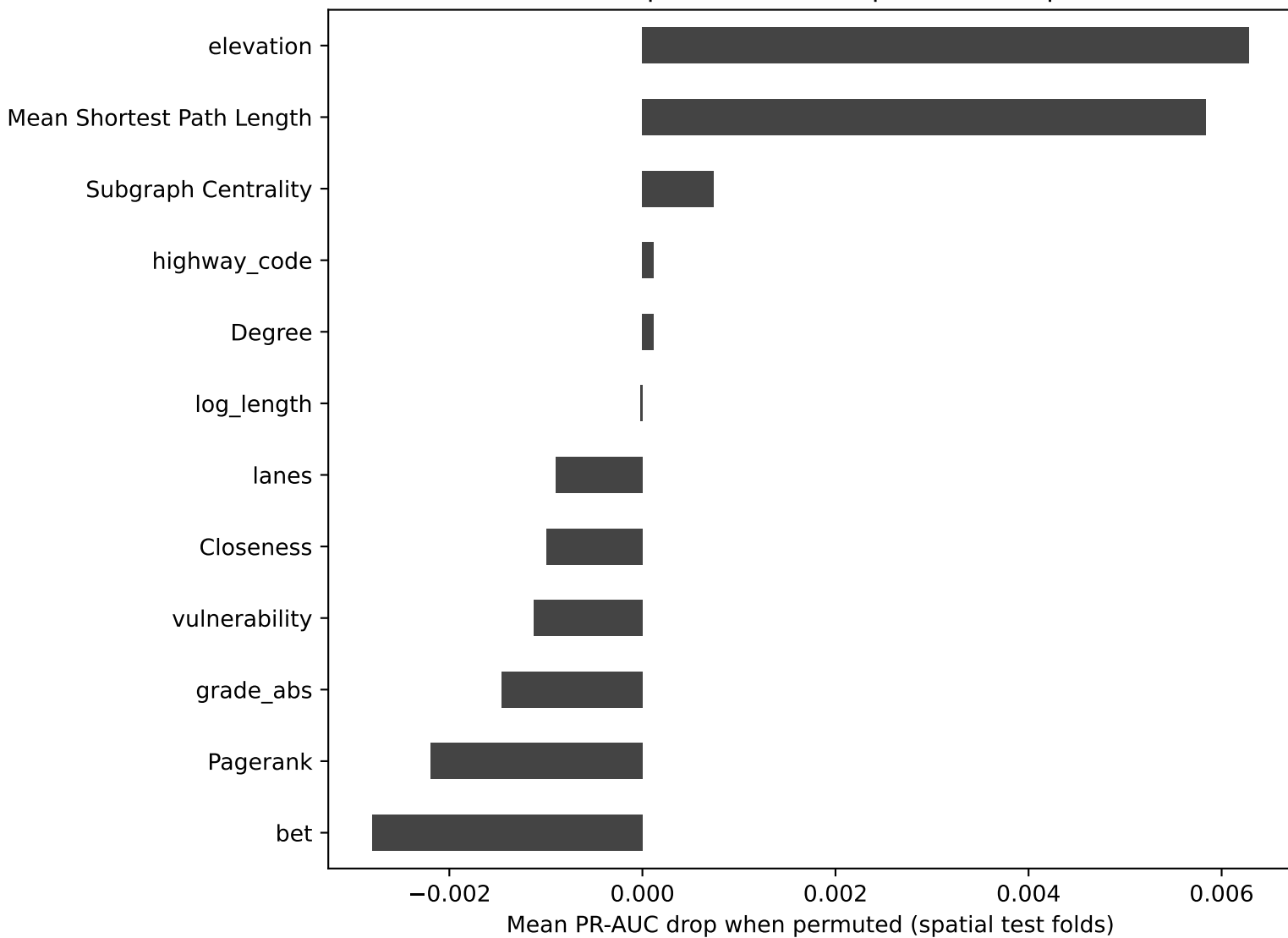
Permutation importance - flood-prone street prediction
