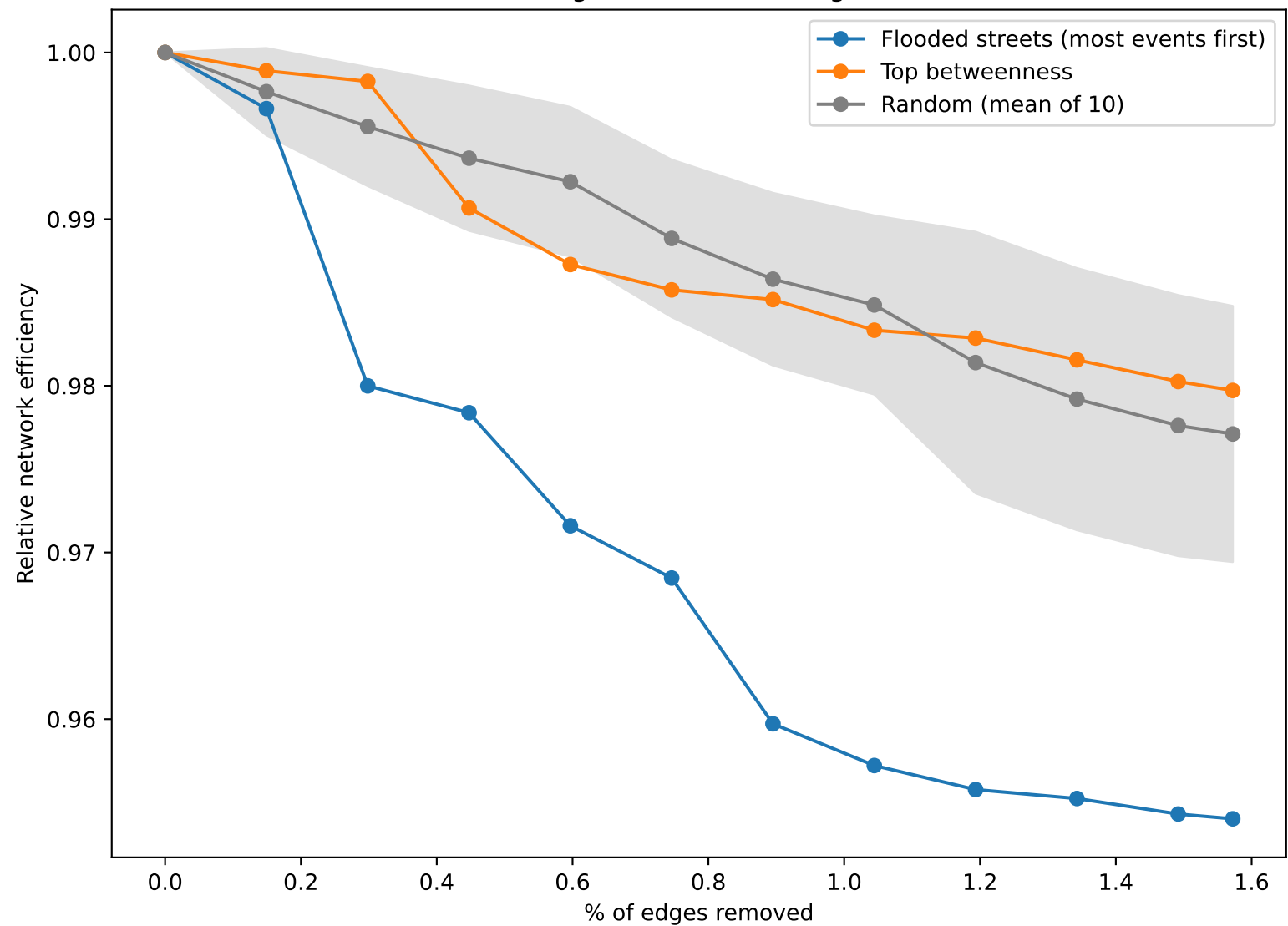
Network degradation under edge removal
