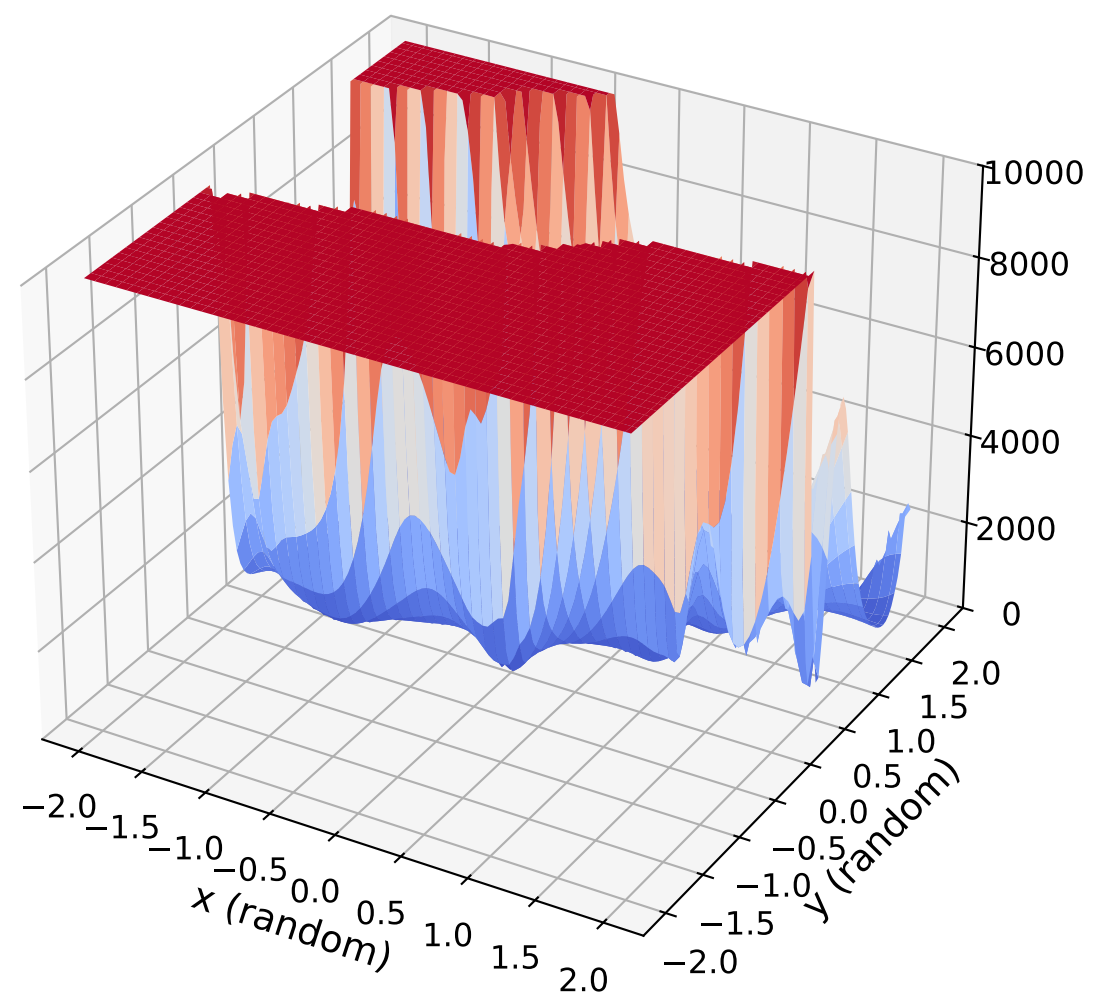
Data-Driven K=1
