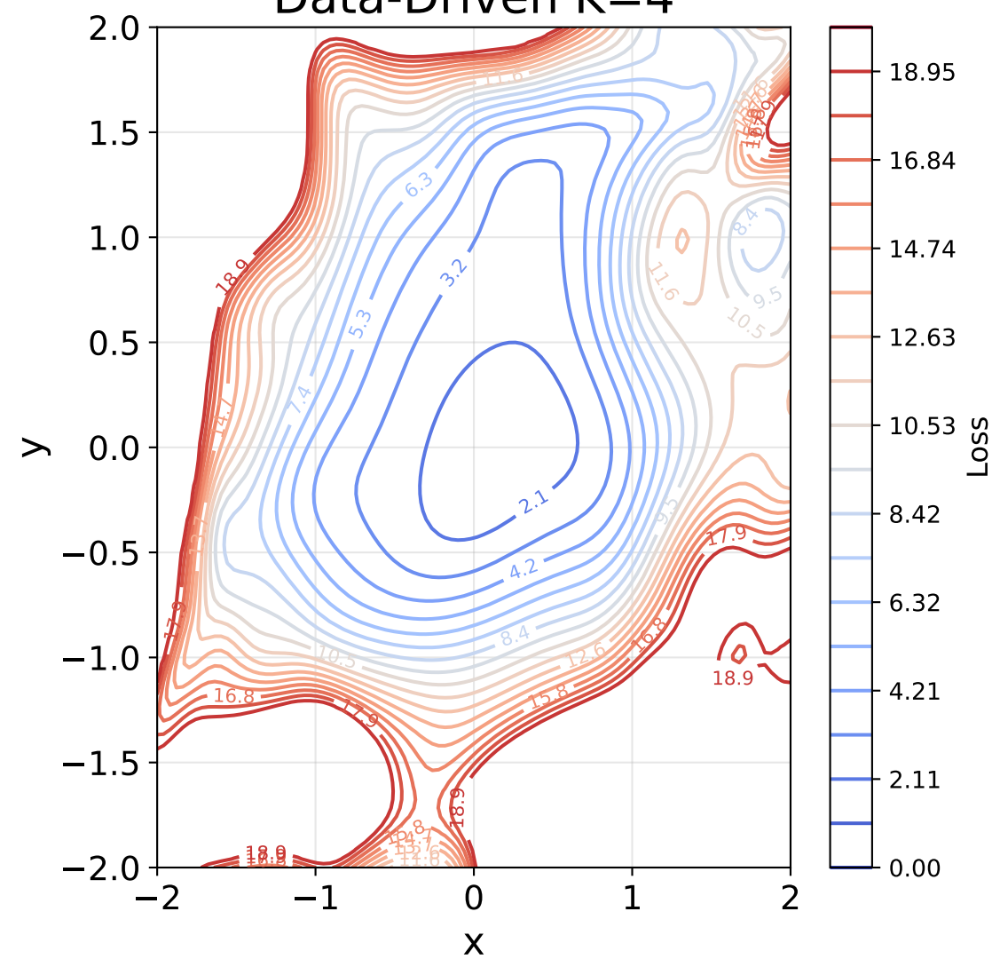
Data-Driven K=4
