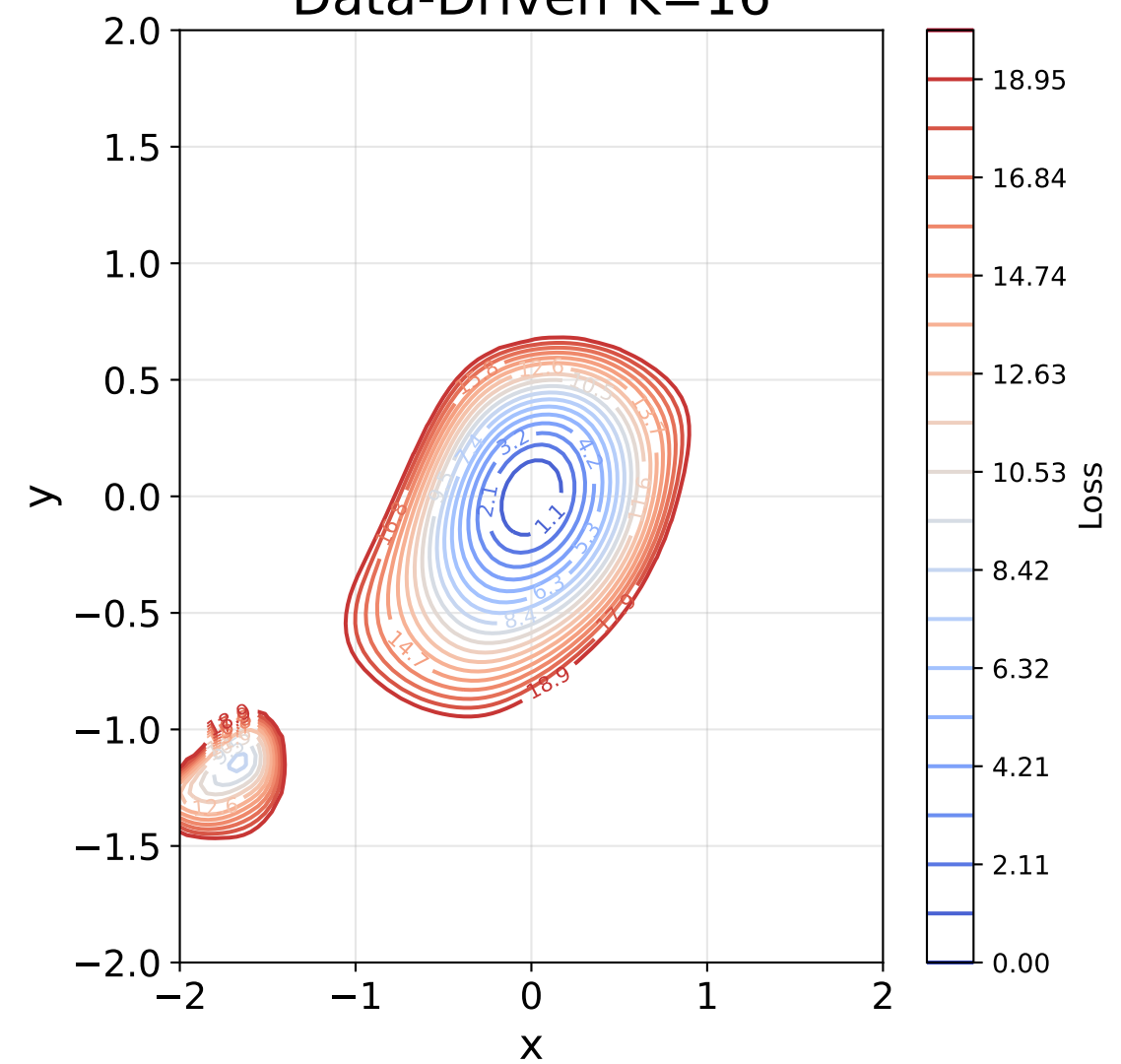
Data-Driven K=16
