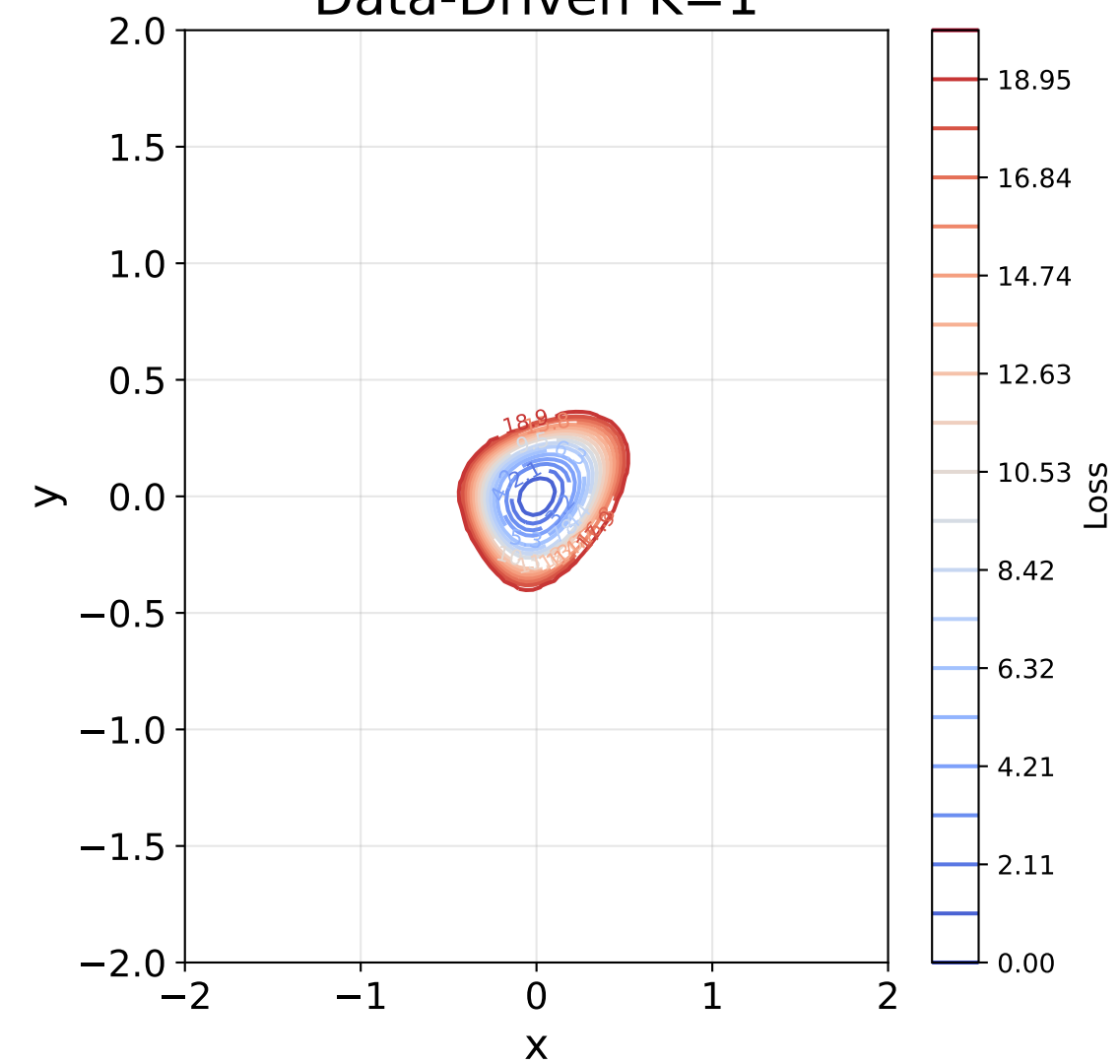
Data-Driven K=1
