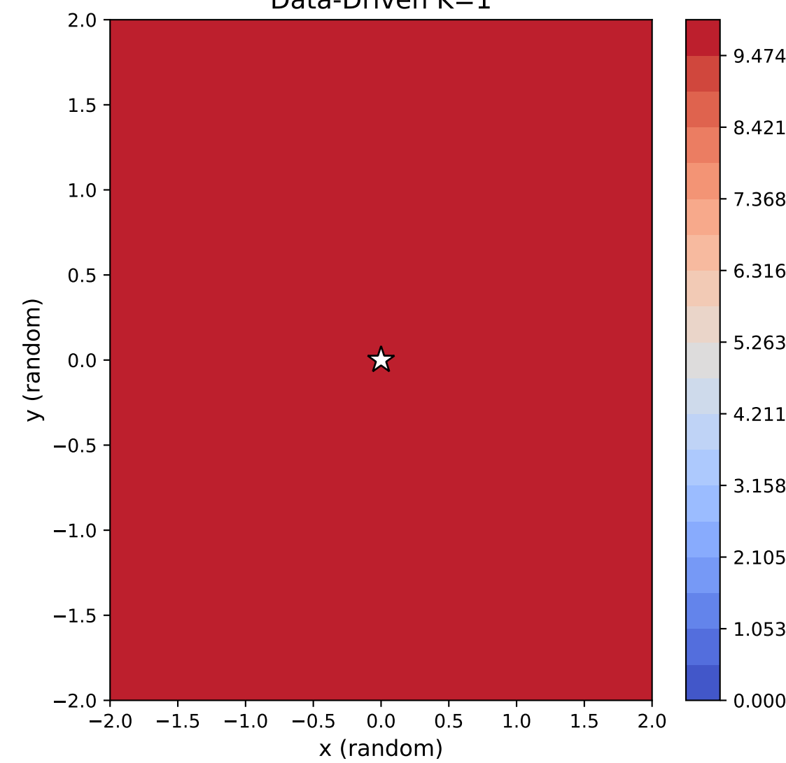
Data-Driven K=1
