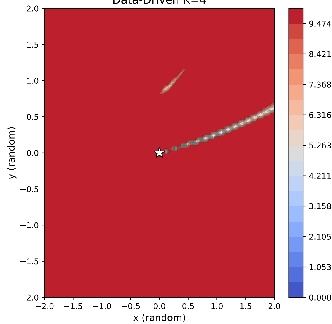
Data-Driven K=4
