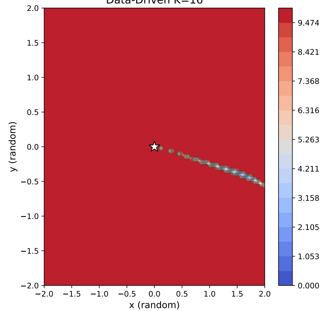
Data-Driven K=16
