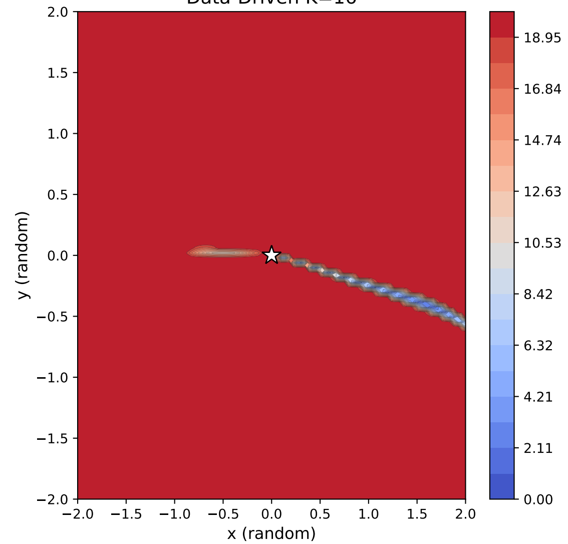
Data-Driven K=16
