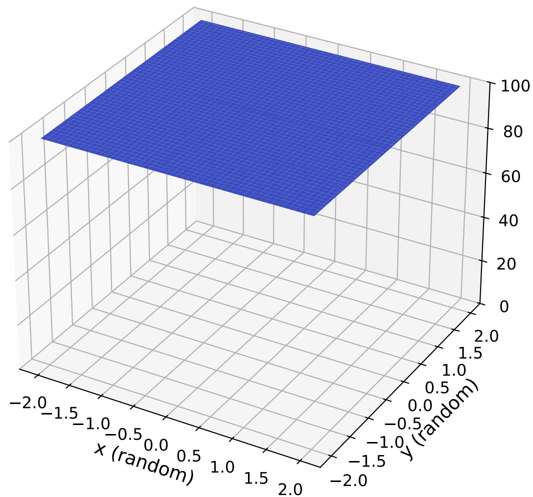
Data-Driven K=1
