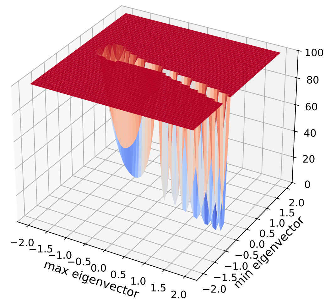
Data-Driven K=16 \lambda_{\max}=3.08\text{e}+02 , \lambda_{\min}=-1.38\text{e}+00
