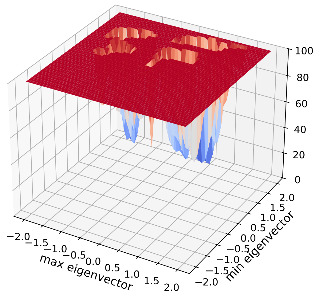
Data-Driven K=1 \lambda_{\max}=8.56\text{e}+03 , \lambda_{\min}=3.43\text{e}+03
