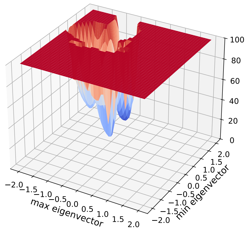
Data-Driven K=4 \lambda_{\max}=4.49\text{e}+02 , \lambda_{\min}=-1.51\text{e}+01
