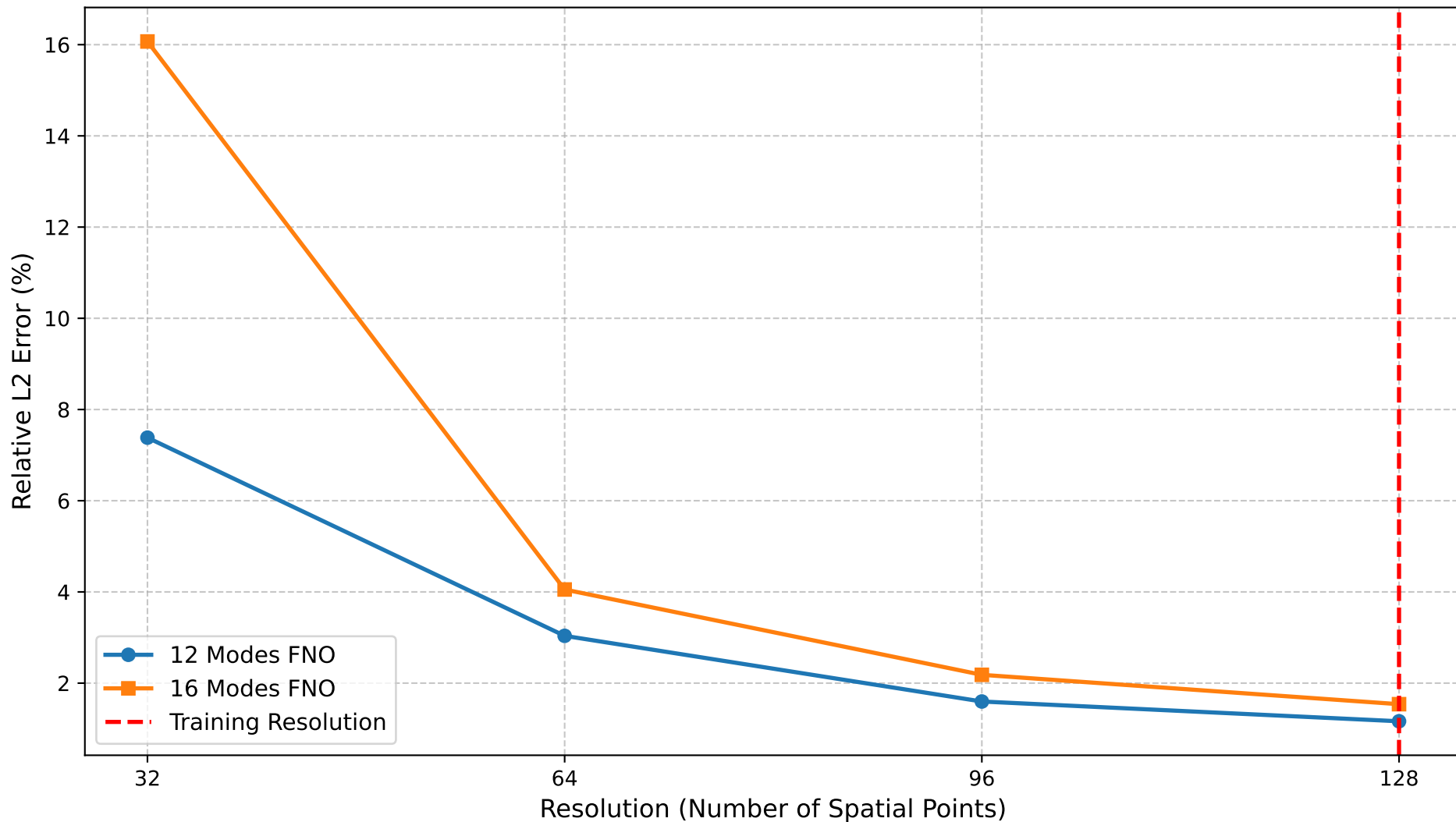
FNO Performance Across Different Resolutions: 12 vs 16 Modes
