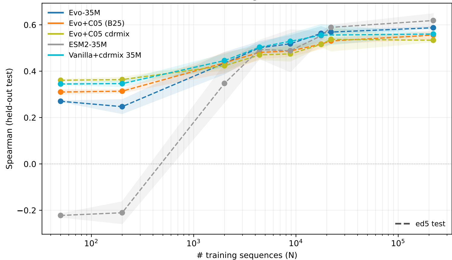
DPO low-data learning curve — ed5 test
