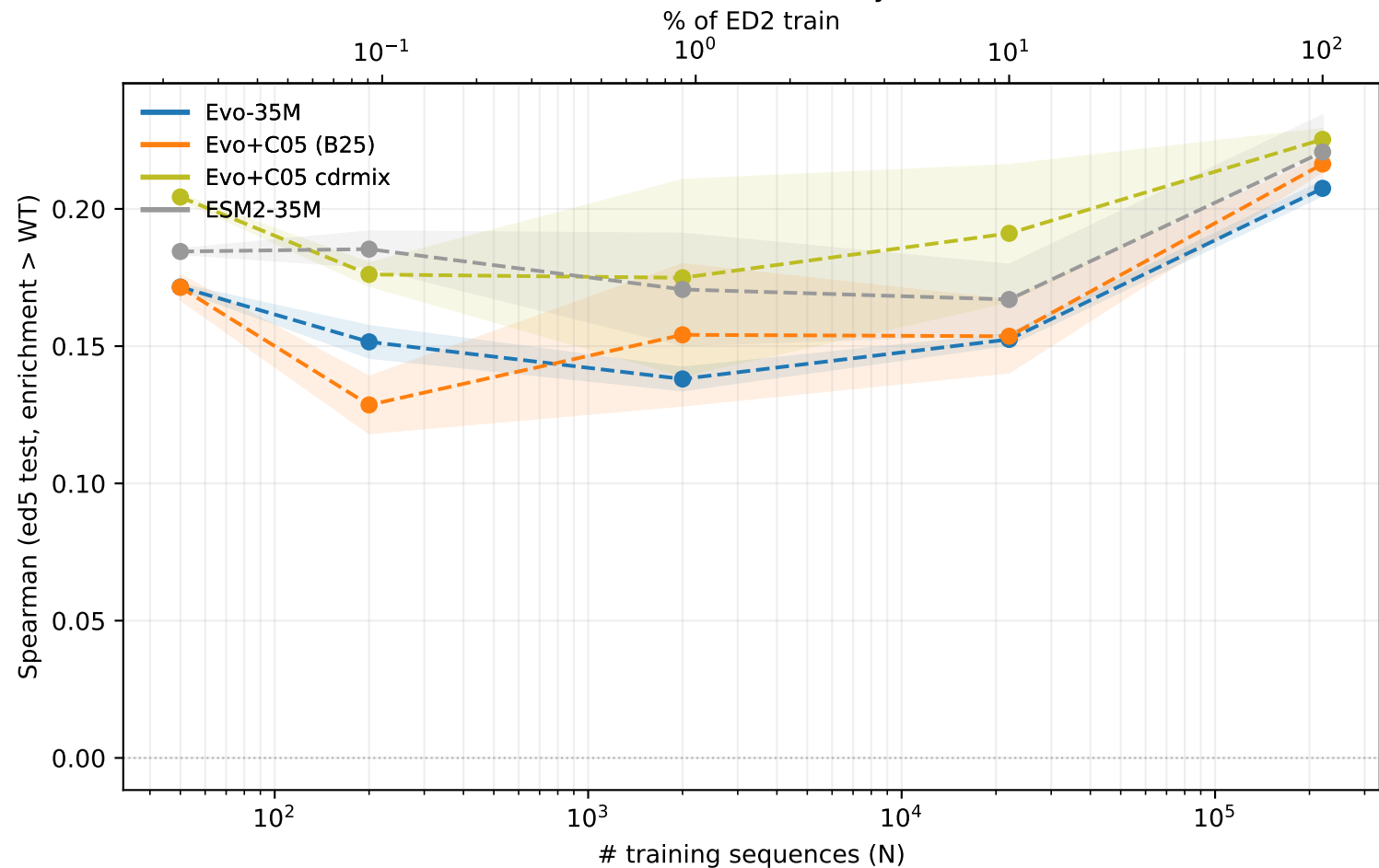
DPO low-data — ed5 test, binders only (enrichment > WT)
