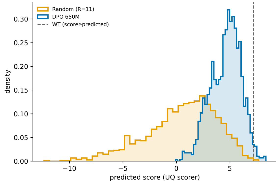
UQ predicted-score distribution (mut \leq 5 )
