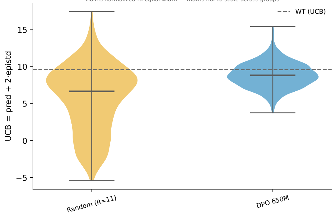
UCB — violin
