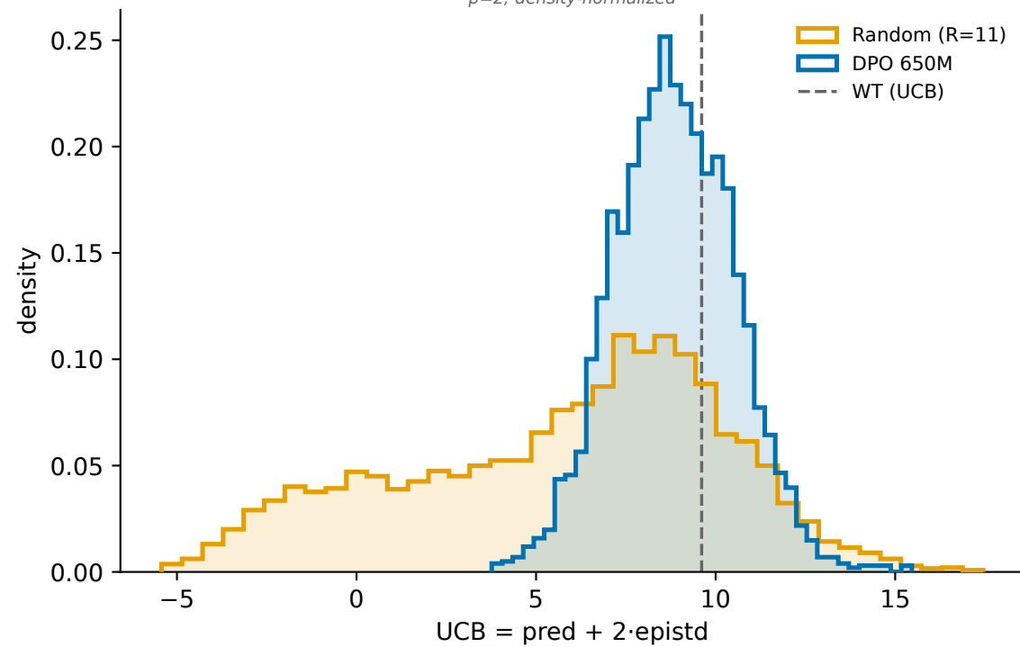
UCB distribution
