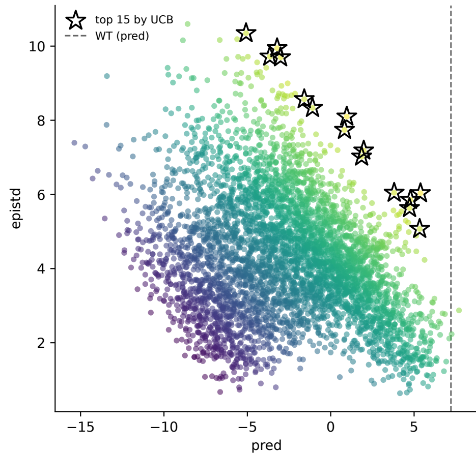
Random (R=11)
