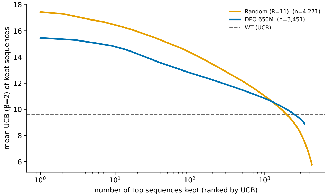
UCB vs selection count (top-N absolute)
