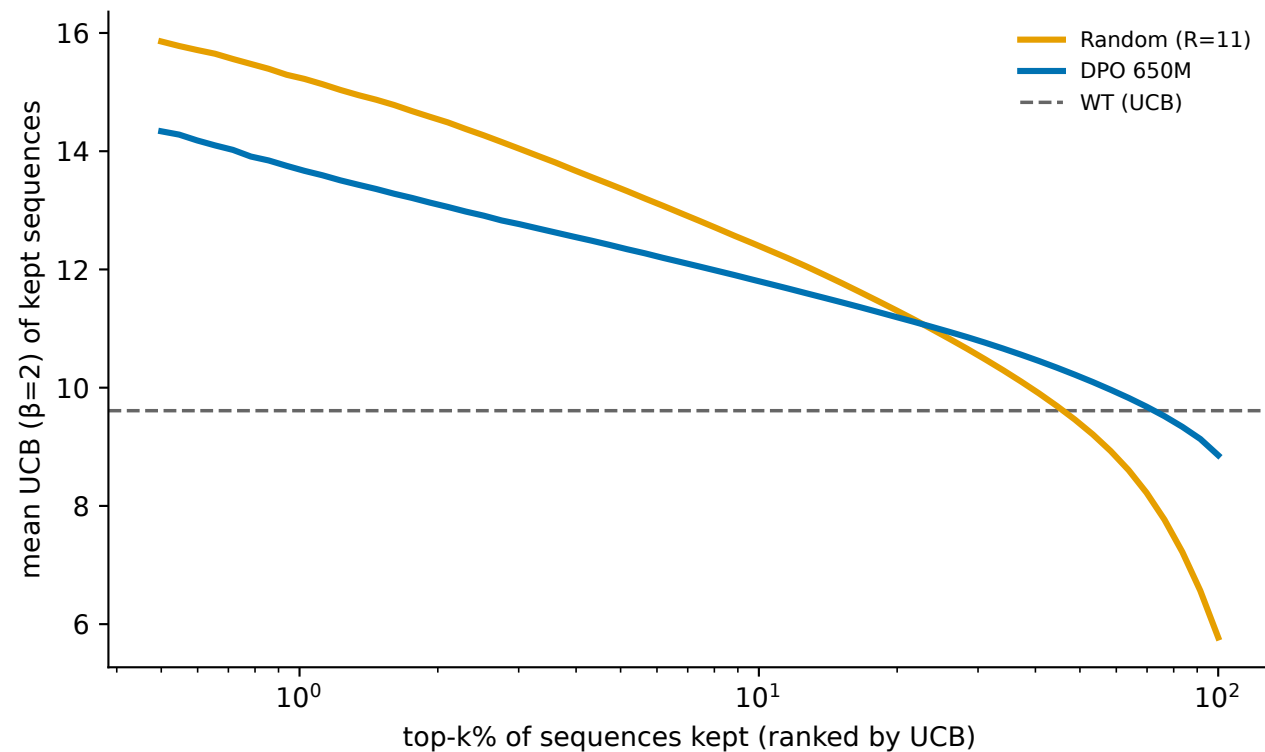
UCB vs selection stringency (top-k%)
