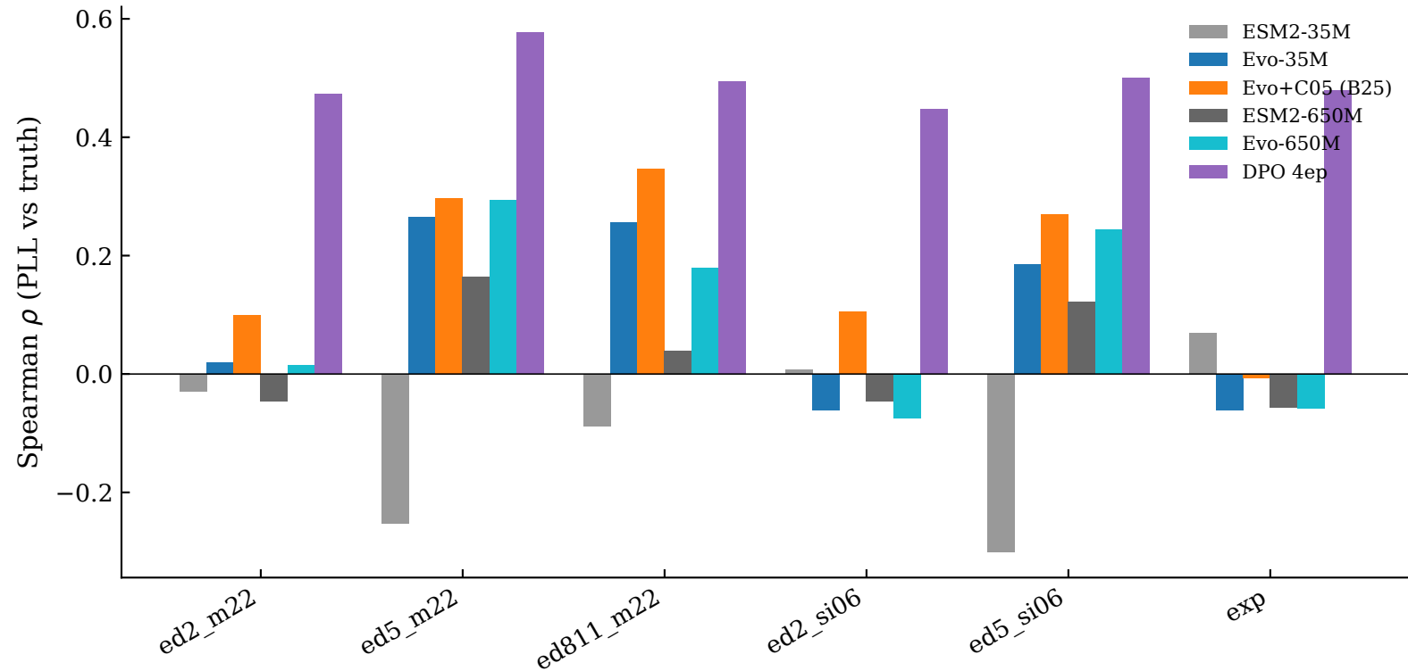
CDR-H3 PLL ranks experimental enrichment
