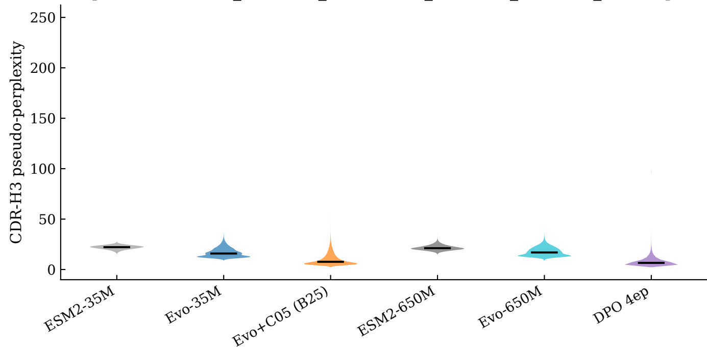
Per-sequence pseudo-perplexity across models (pooled from: ed2_m22, ed5_m22, ed811_m22, ed2_si06, ed5_si06, exp)
