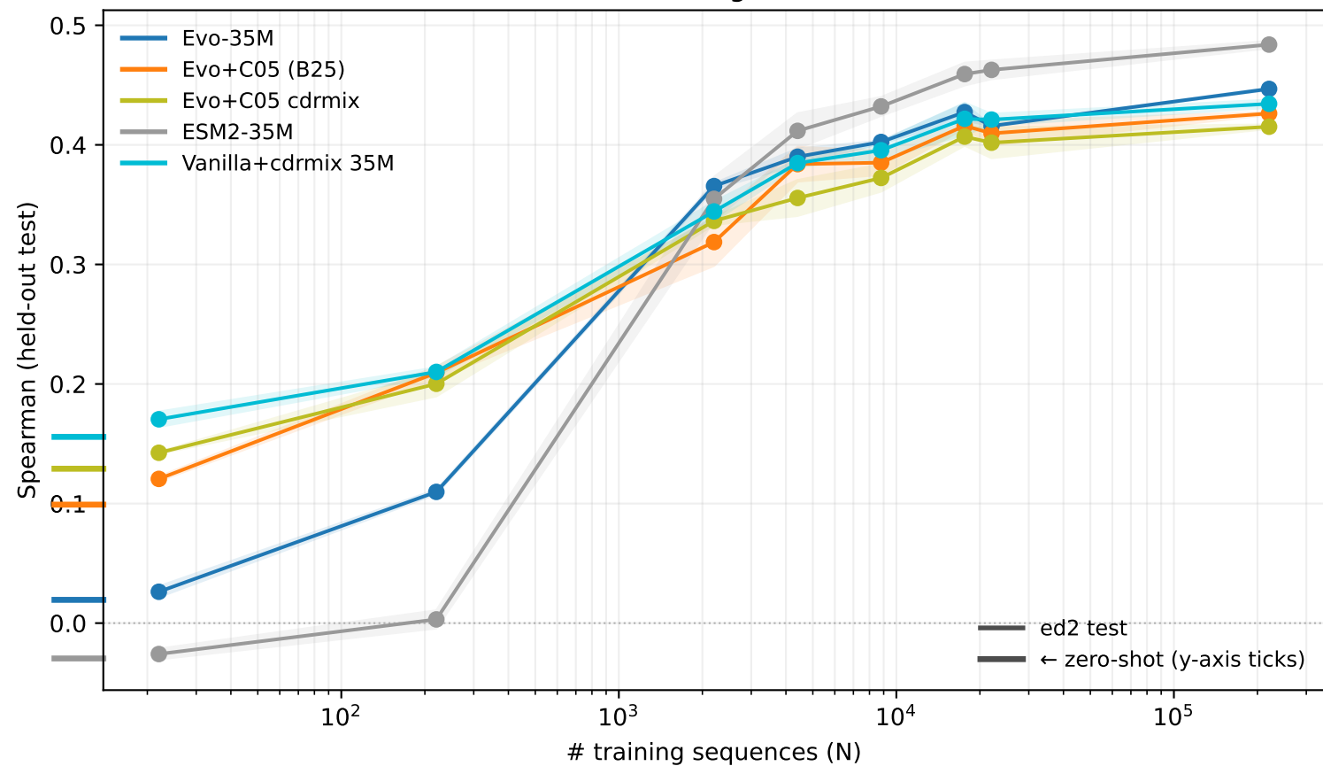
DPO low-data learning curve — ed2 test
