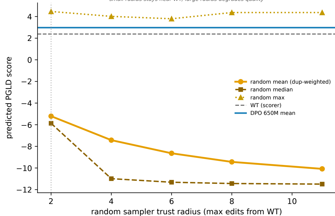
PGLD score vs trust radius
