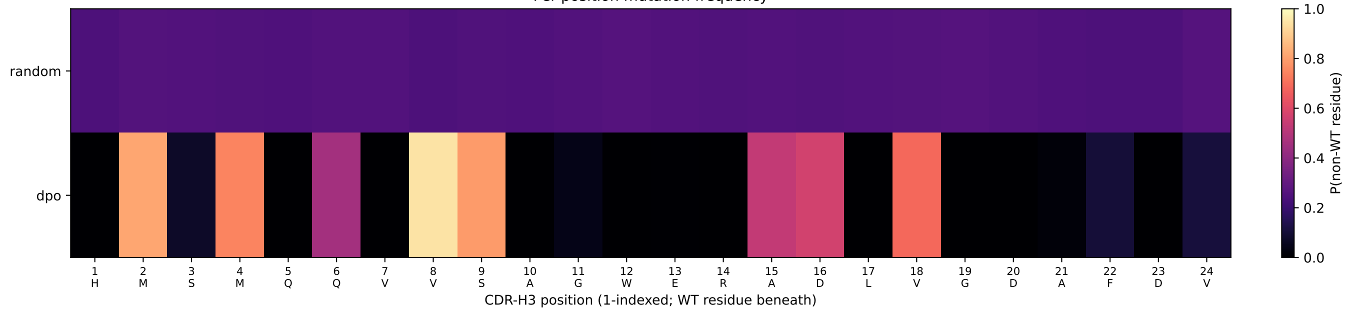
Per-position mutation frequency
