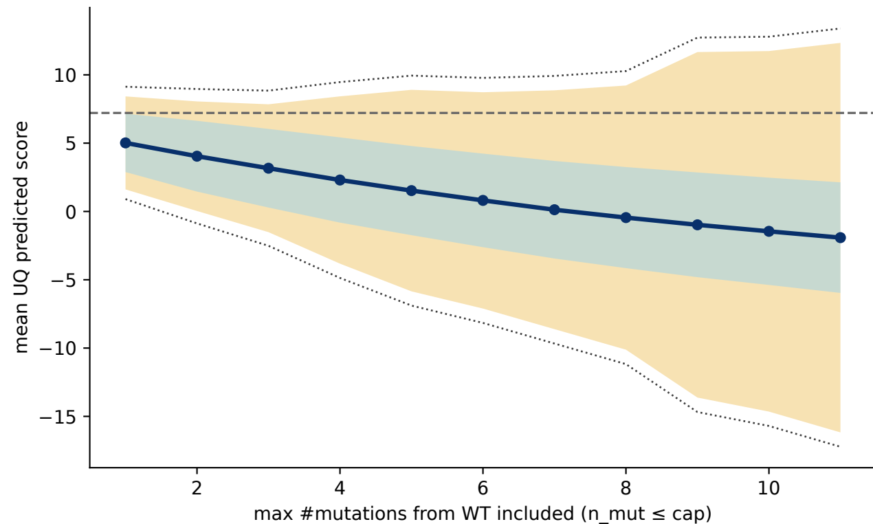
Random (R=11)
