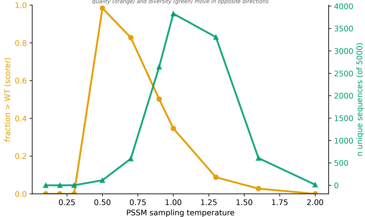
Score-vs-diversity trade-off
