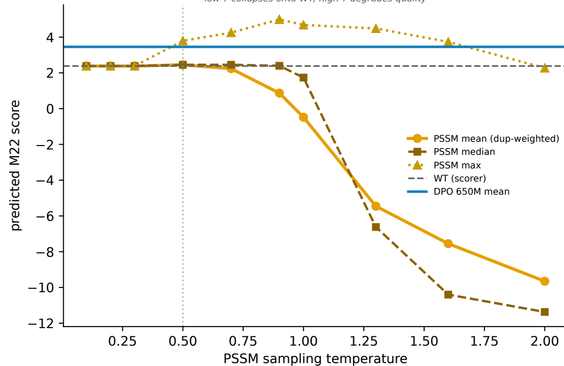
M22 score vs PSSM temperature
