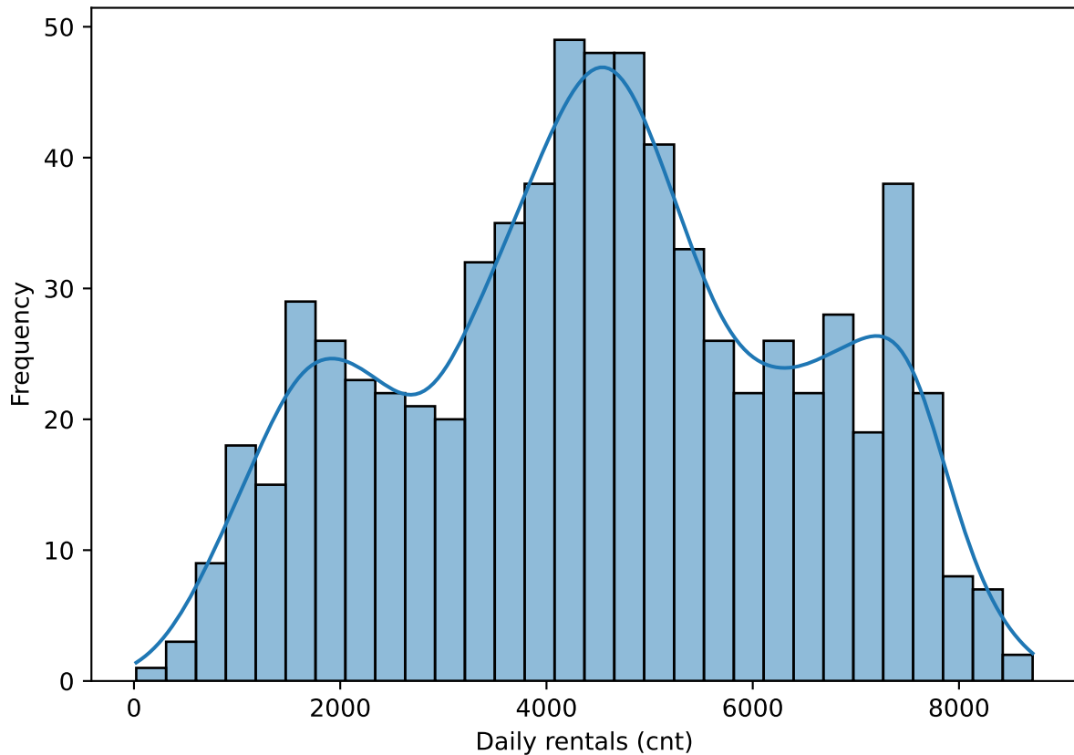
Distribution of Daily Bike Rentals
