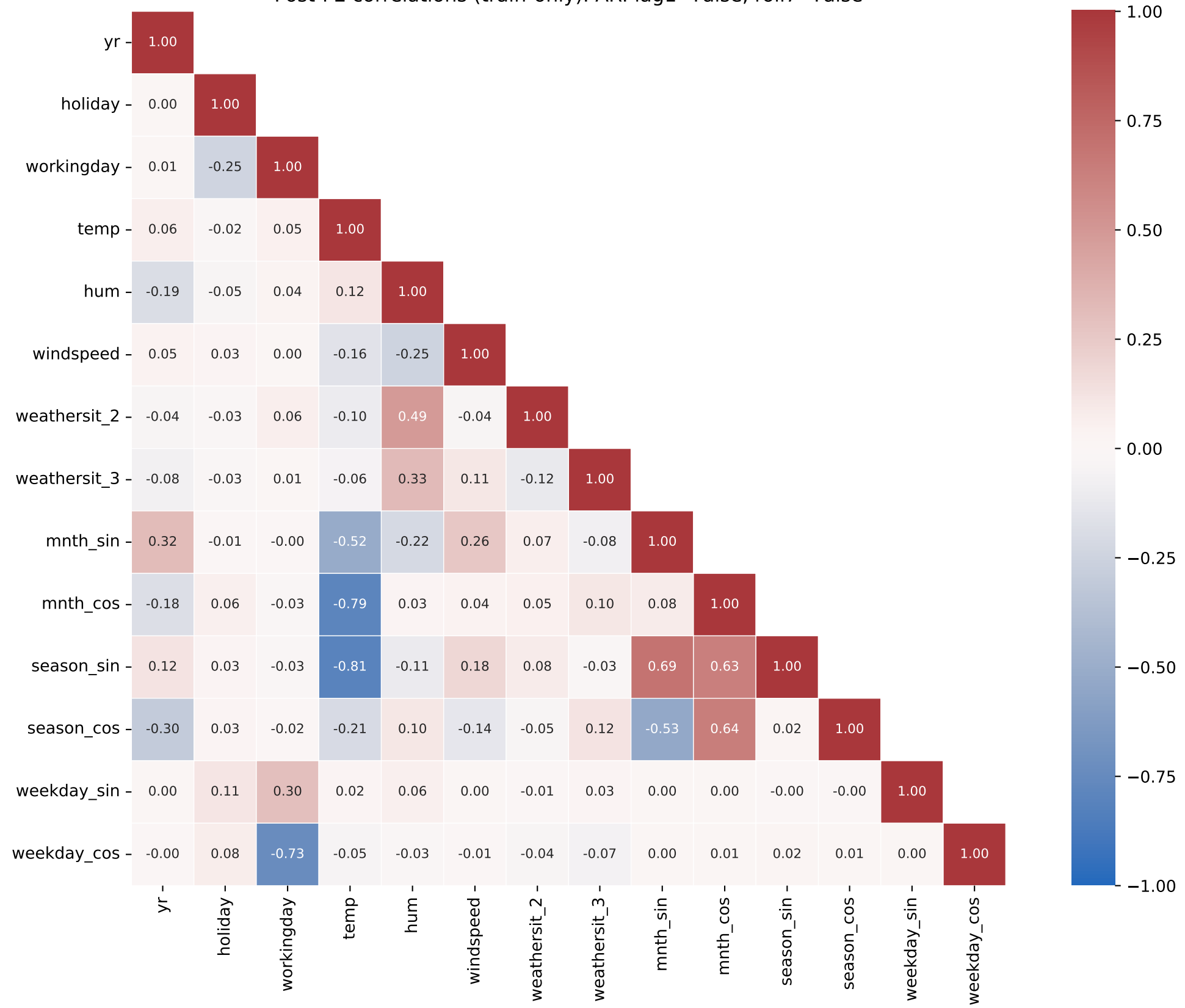
Post-FE correlations (train-only). AR: lag1=False, roll7=False
