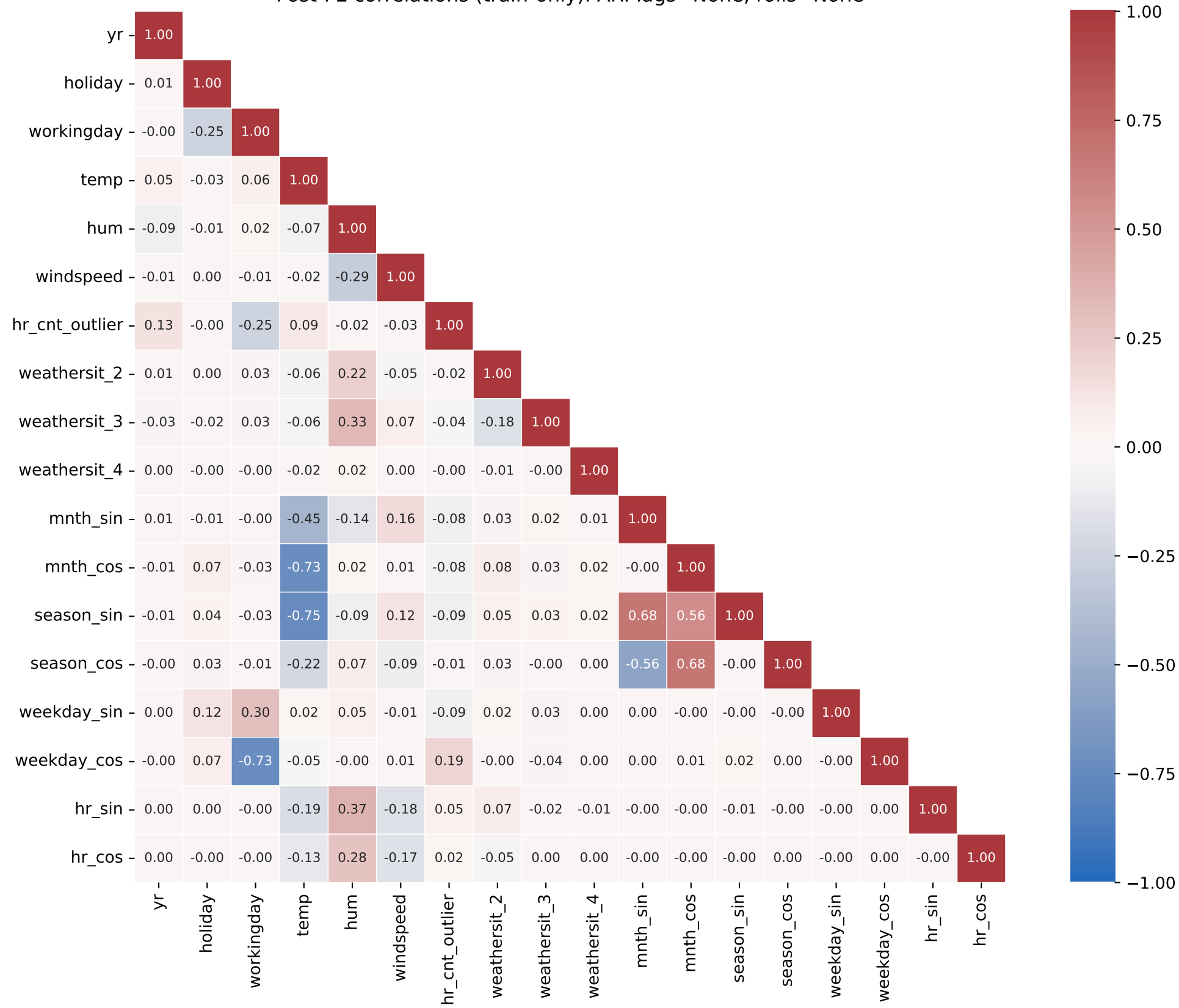
Post-FE correlations (train-only). AR: lags=None, rolls=None
